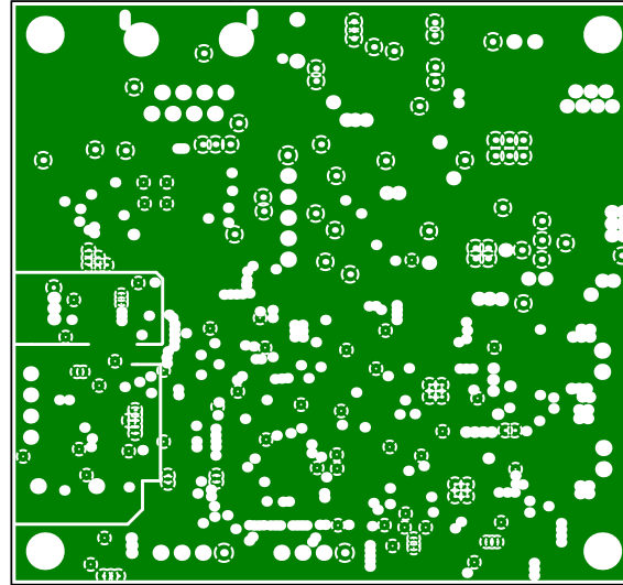
GND (Scale 1:1)
